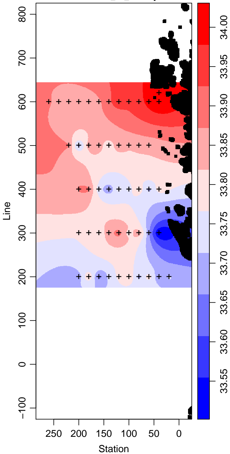
LMG04-01_45_Salinity
