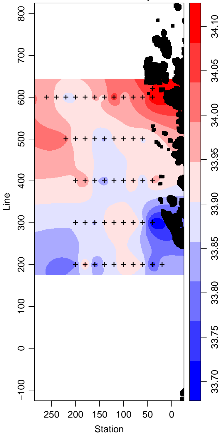
LMG04-01_60_Salinity
