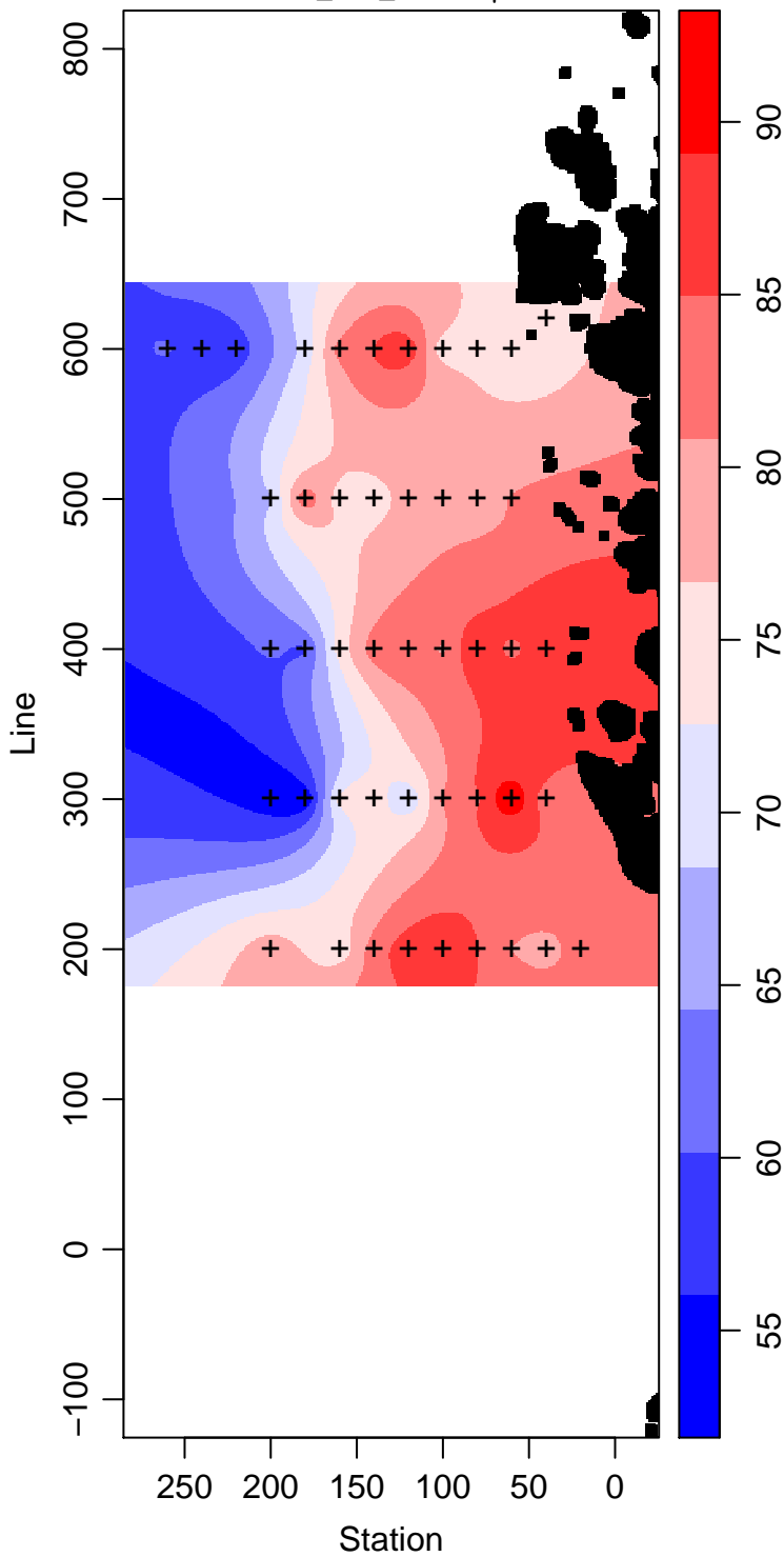
LMG04-01_100_Silicate \mu\text{ mol L}^{-1}
