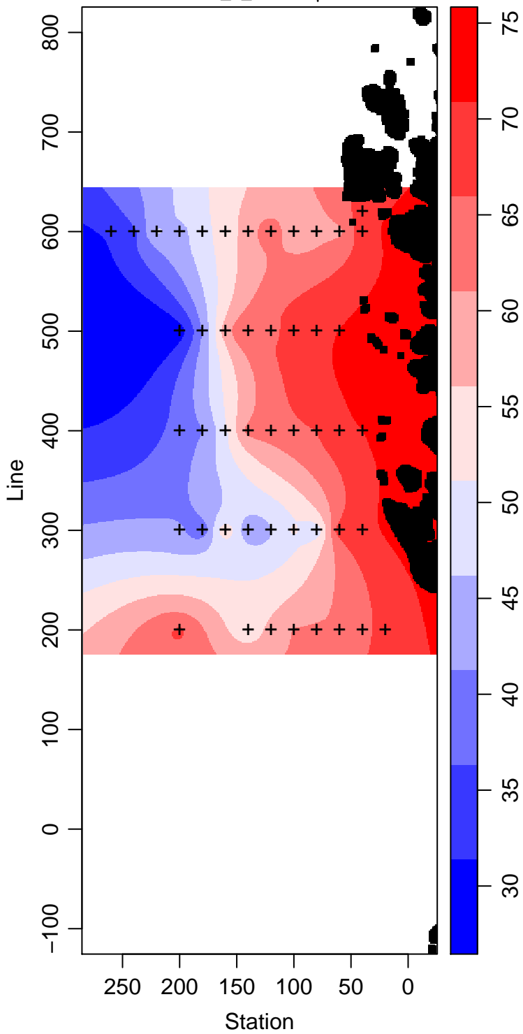
LMG04-01_1_Silicate \mu\text{ mol L}^{-1}
