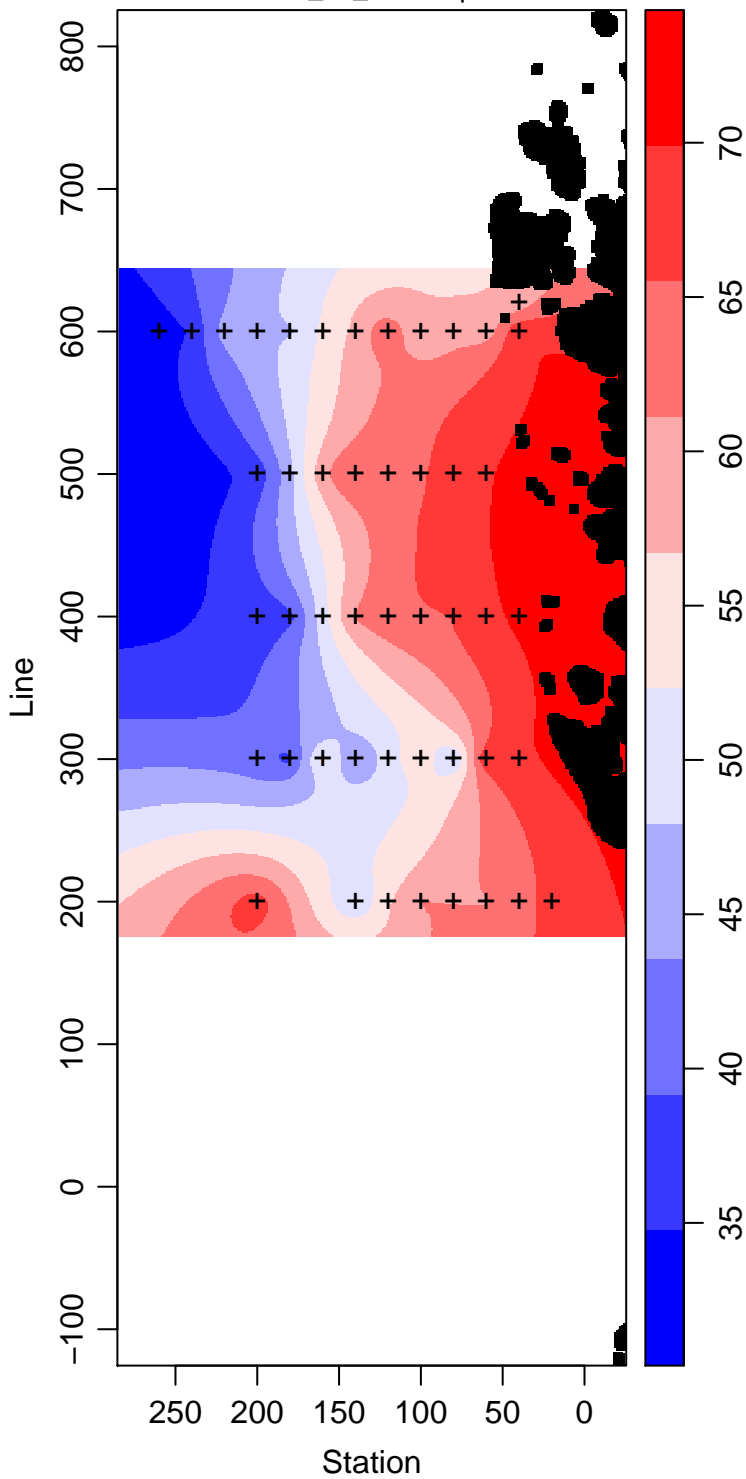
LMG04-01_20_Silicate \mu\text{ mol L}^{-1}
