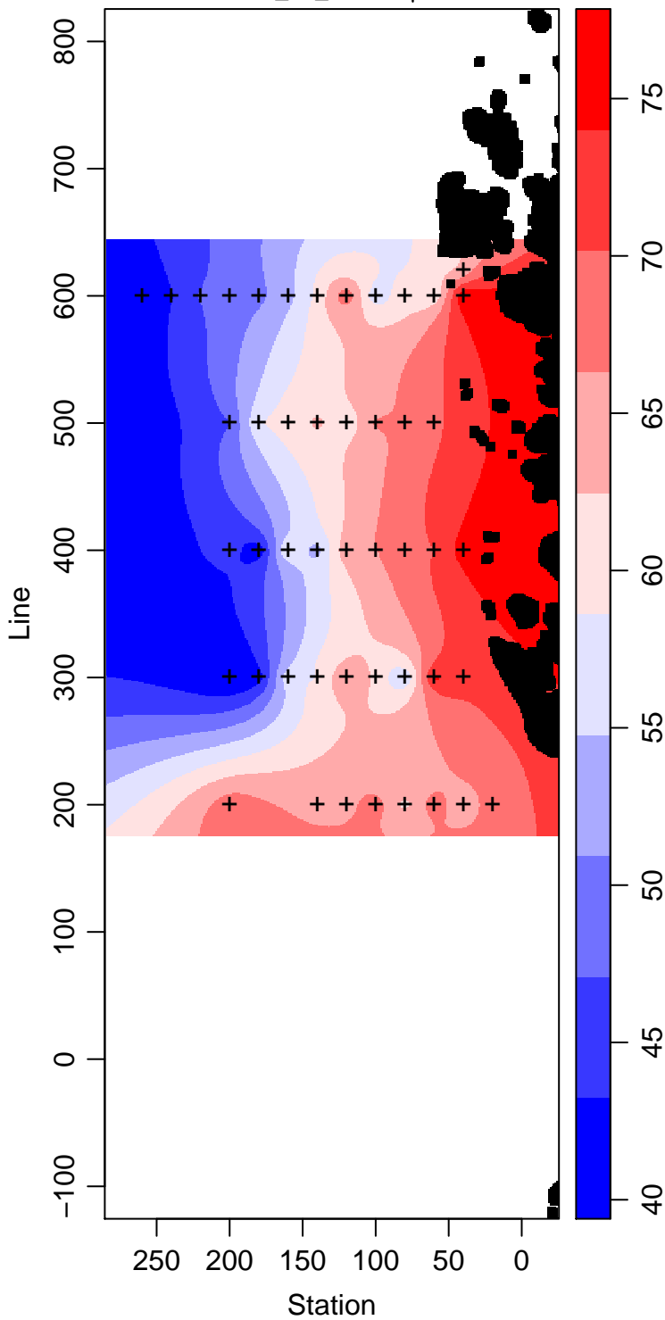
LMG04-01_40_Silicate \mu\text{ mol L}^{-1}
