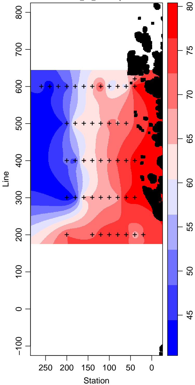
LMG04-01_55_Silicate \mu\text{ mol L}^{-1}
