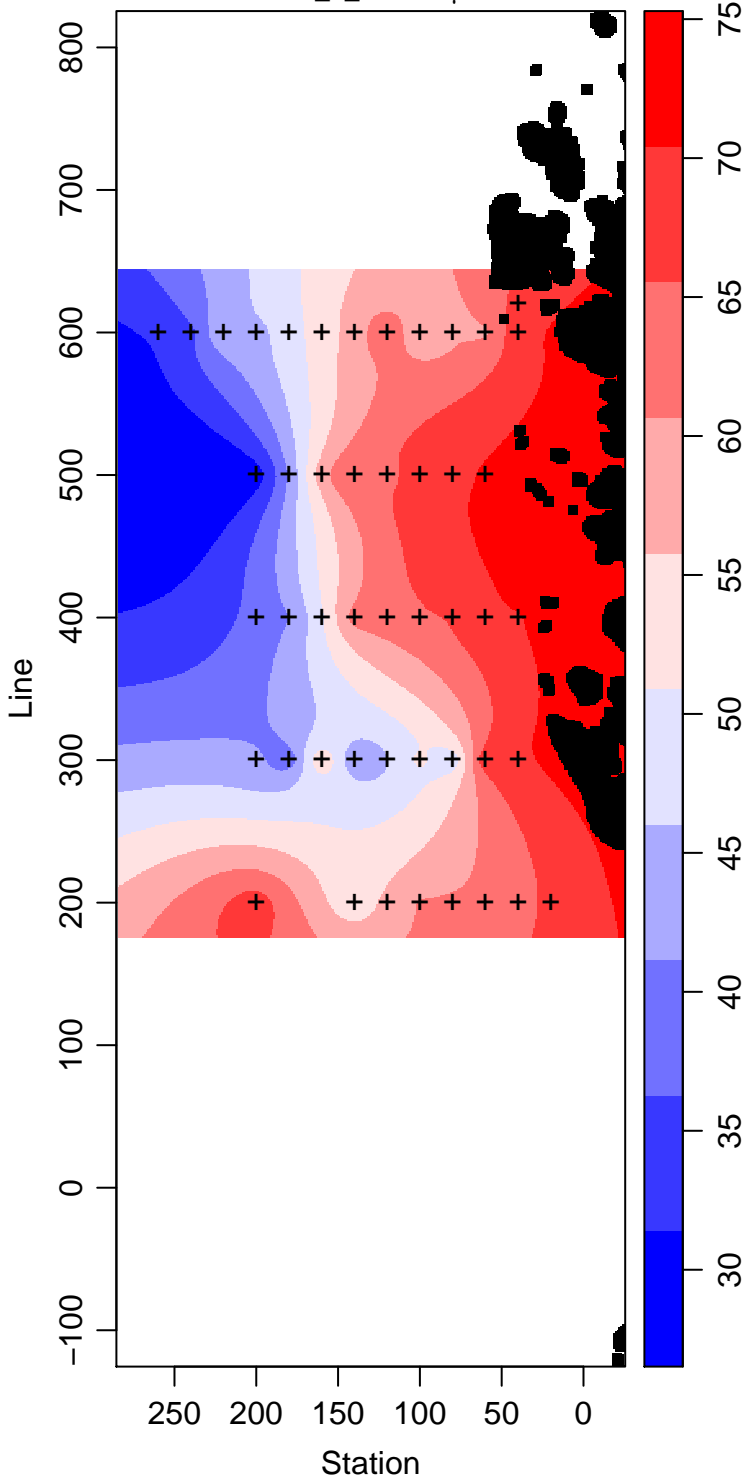
LMG04-01_5_Silicate \mu\text{ mol L}^{-1}
