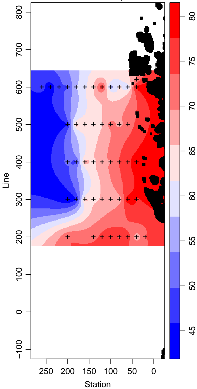
LMG04-01_60_Silicate \mu\text{ mol L}^{-1}
