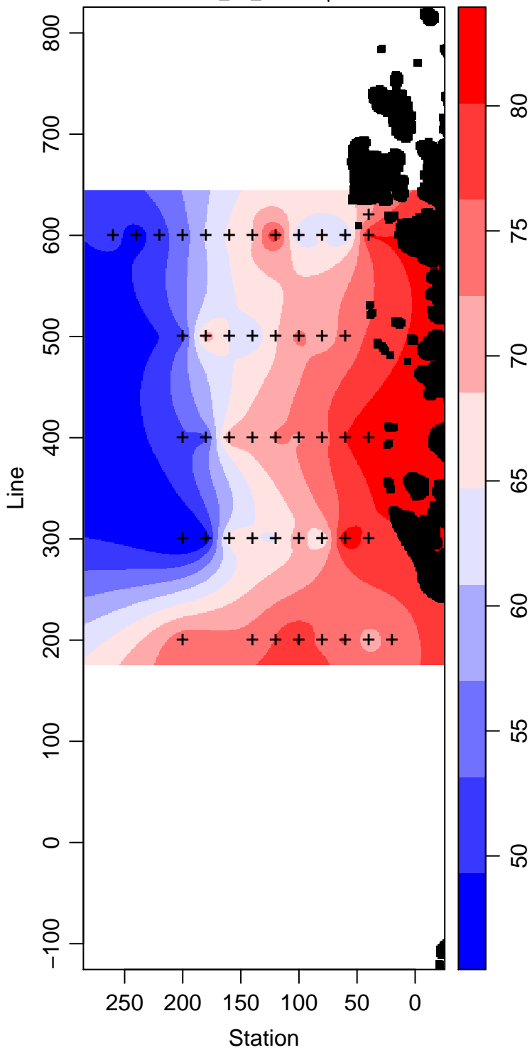
LMG04-01_70_Silicate \mu\text{ mol L}^{-1}
