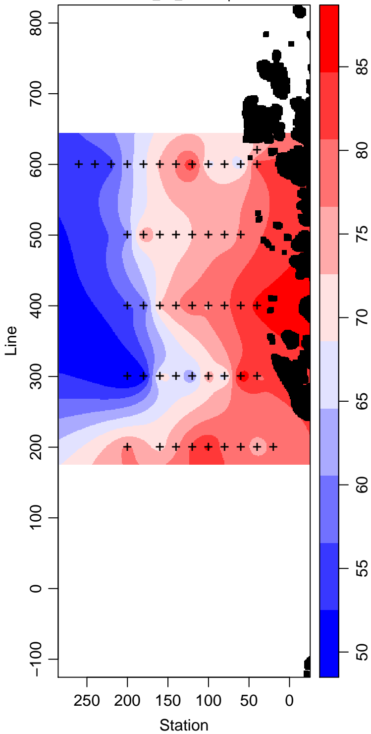
LMG04-01_85_Silicate \mu\text{ mol L}^{-1}
