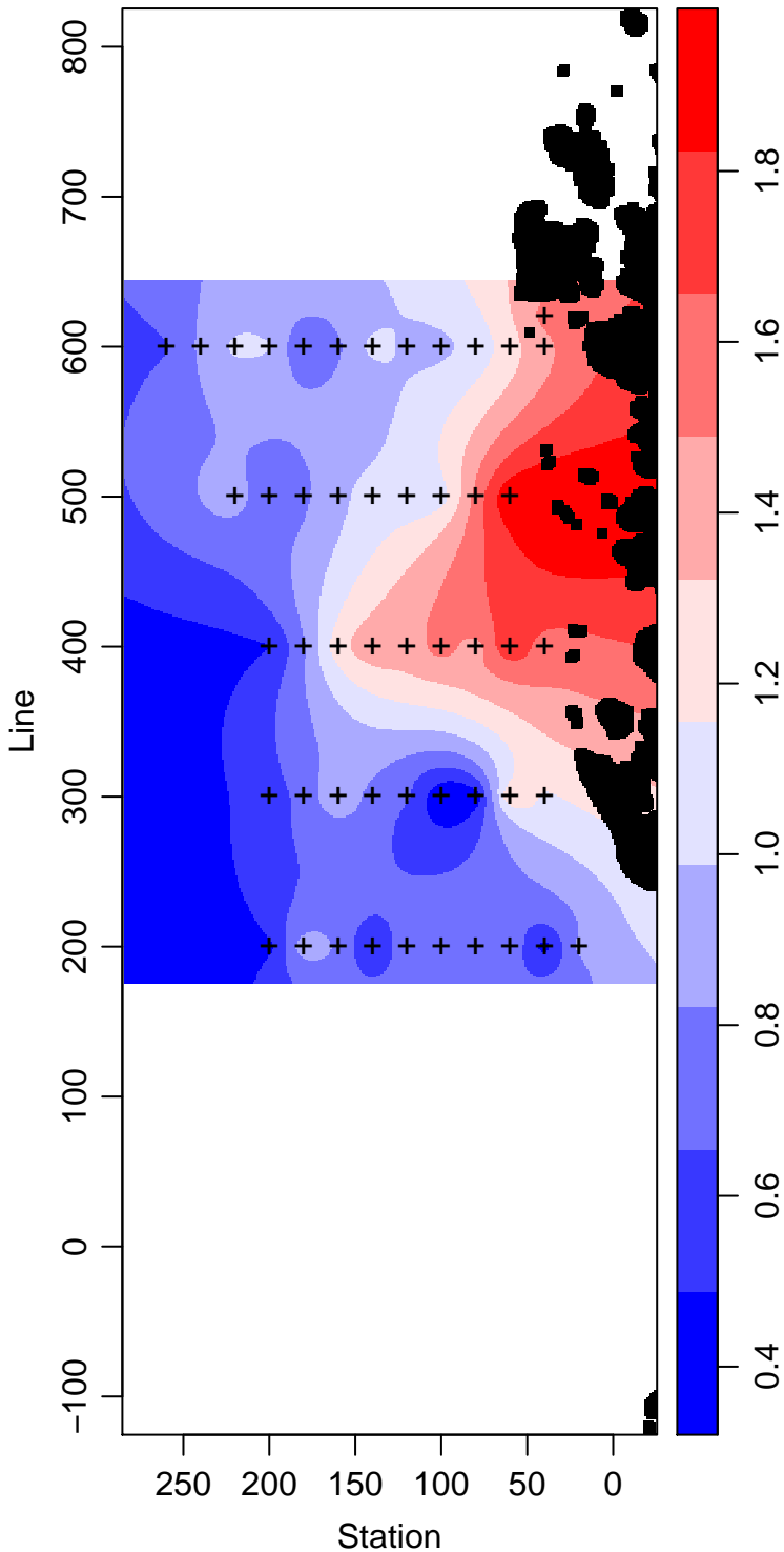
LMG04-01_15_Temperature ° Celsius
