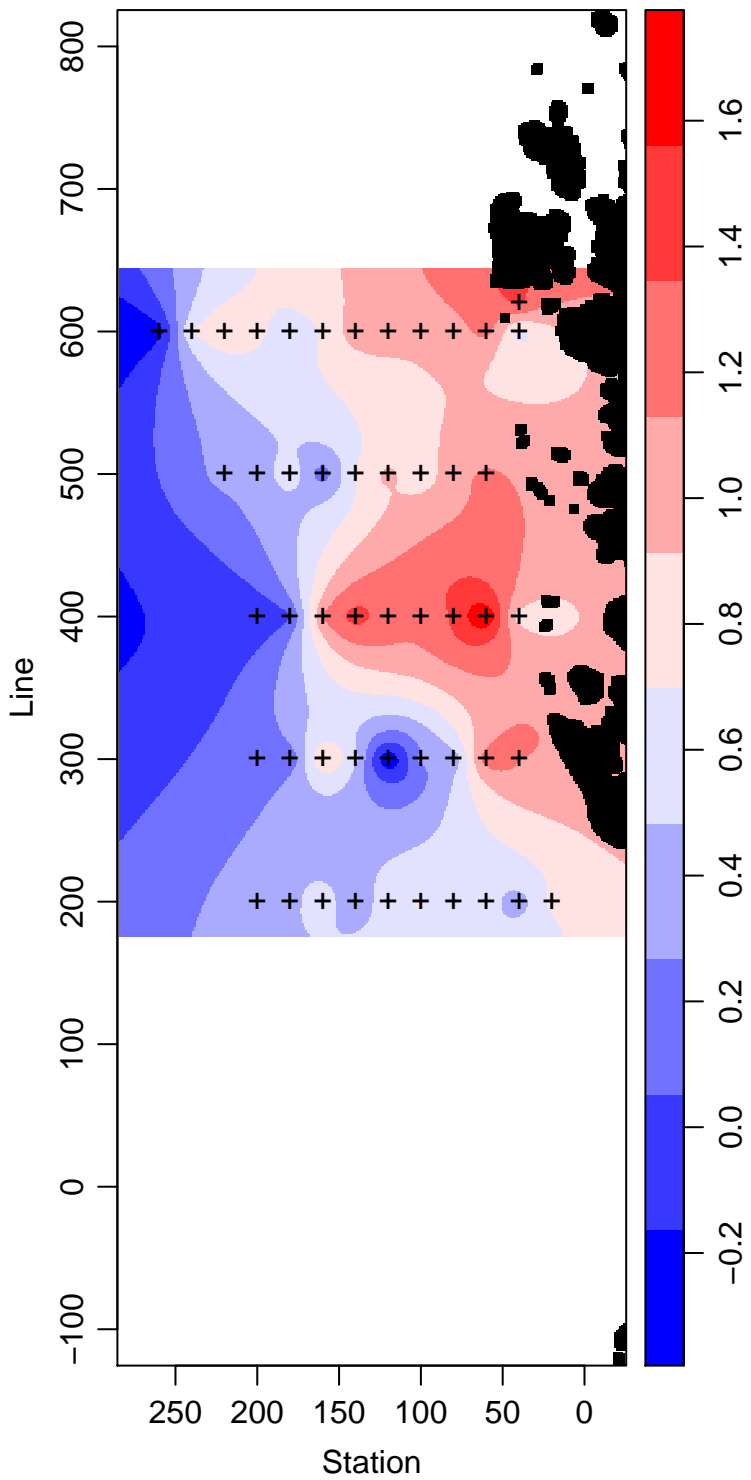
LMG04-01_25_Temperature ° Celsius
