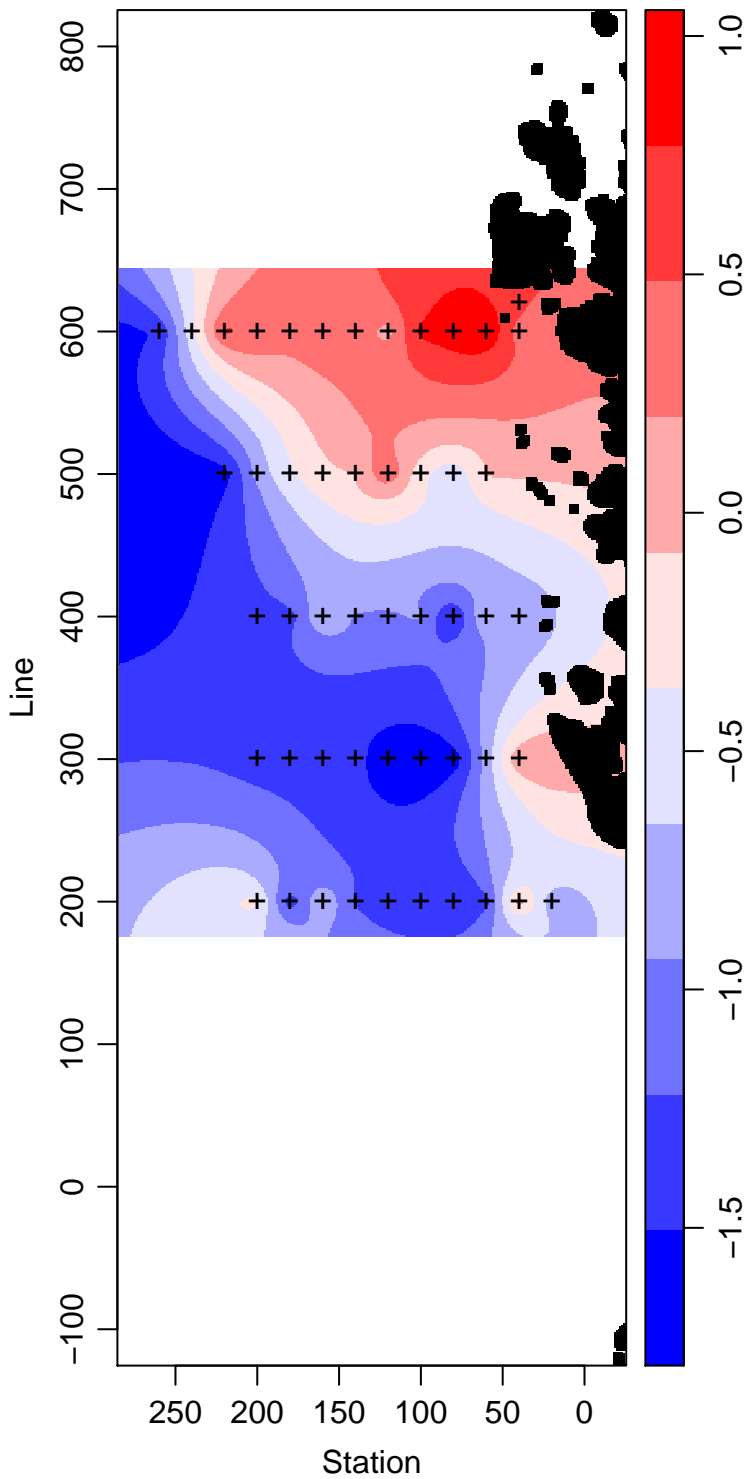
LMG04-01_50_Temperature ° Celsius
