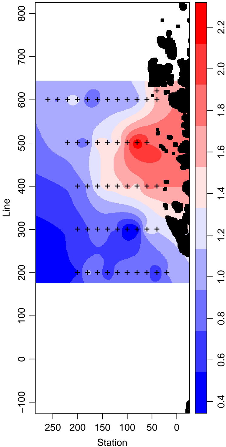
LMG04-01_5_Temperature ° Celsius
