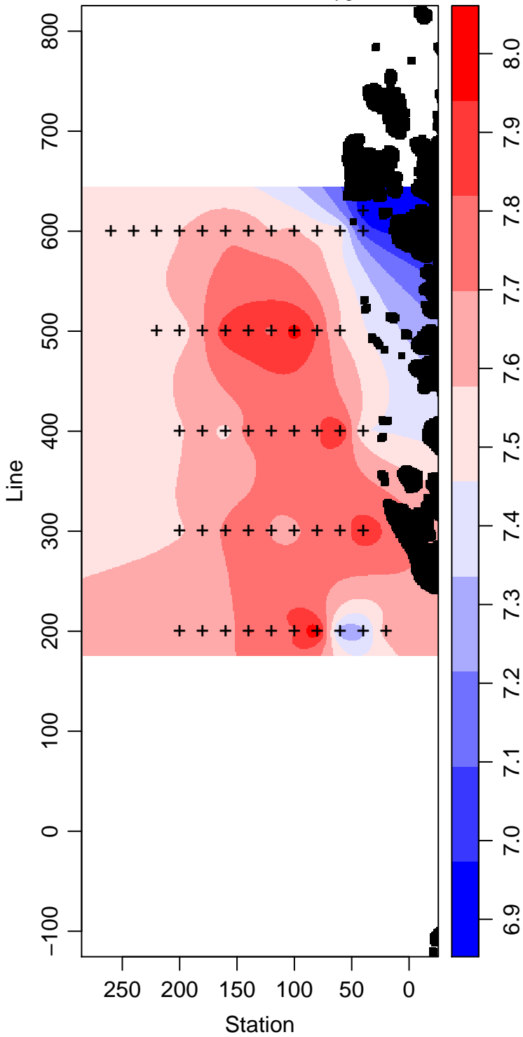
LMG05-01_15_Dissolved.Oxygen ml L -1
