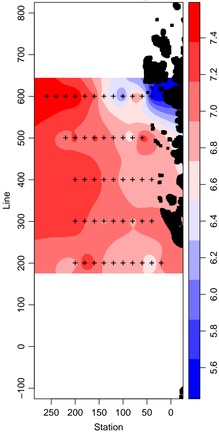
LMG05-01_55_Dissolved.Oxygen ml L -1
