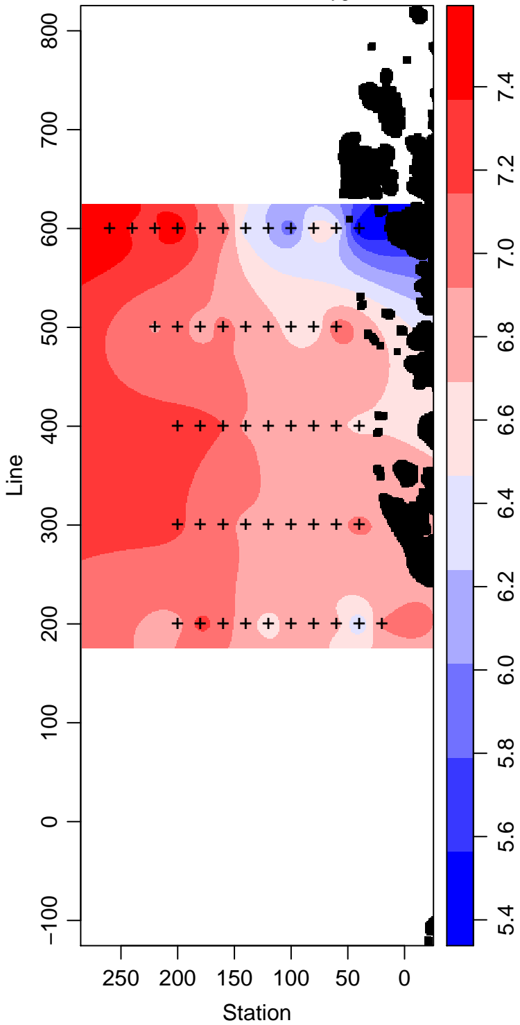
LMG05-01_60_Dissolved.Oxygen ml L -1
