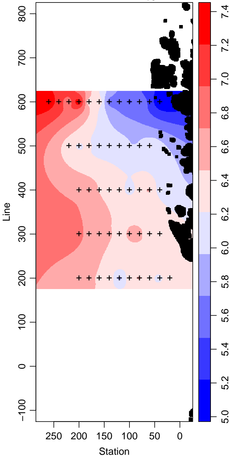
LMG05-01_80_Dissolved.Oxygen ml L -1
