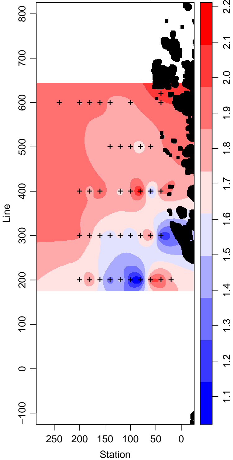
LMG05-01_10_Phosphate \mu\text{ mol L}^{-1}
