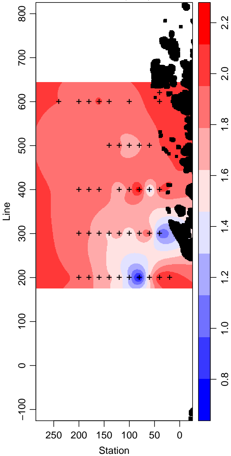
LMG05-01_15_Phosphate \mu\text{ mol L}^{-1}
