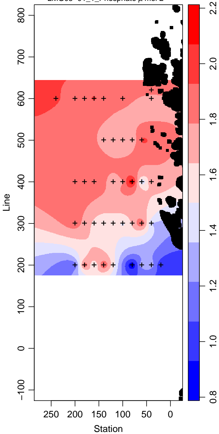
LMG05-01_1_Phosphate \mu\text{ mol L}^{-1}
