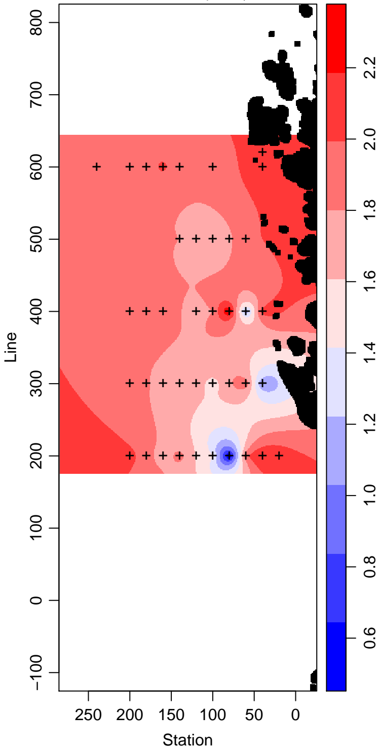
LMG05-01_20_Phosphate \mu\text{ mol L}^{-1}
