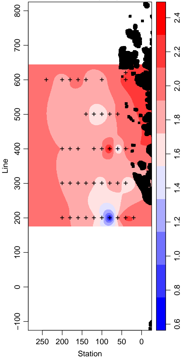
LMG05-01_25_Phosphate \mu\text{ mol L}^{-1}
