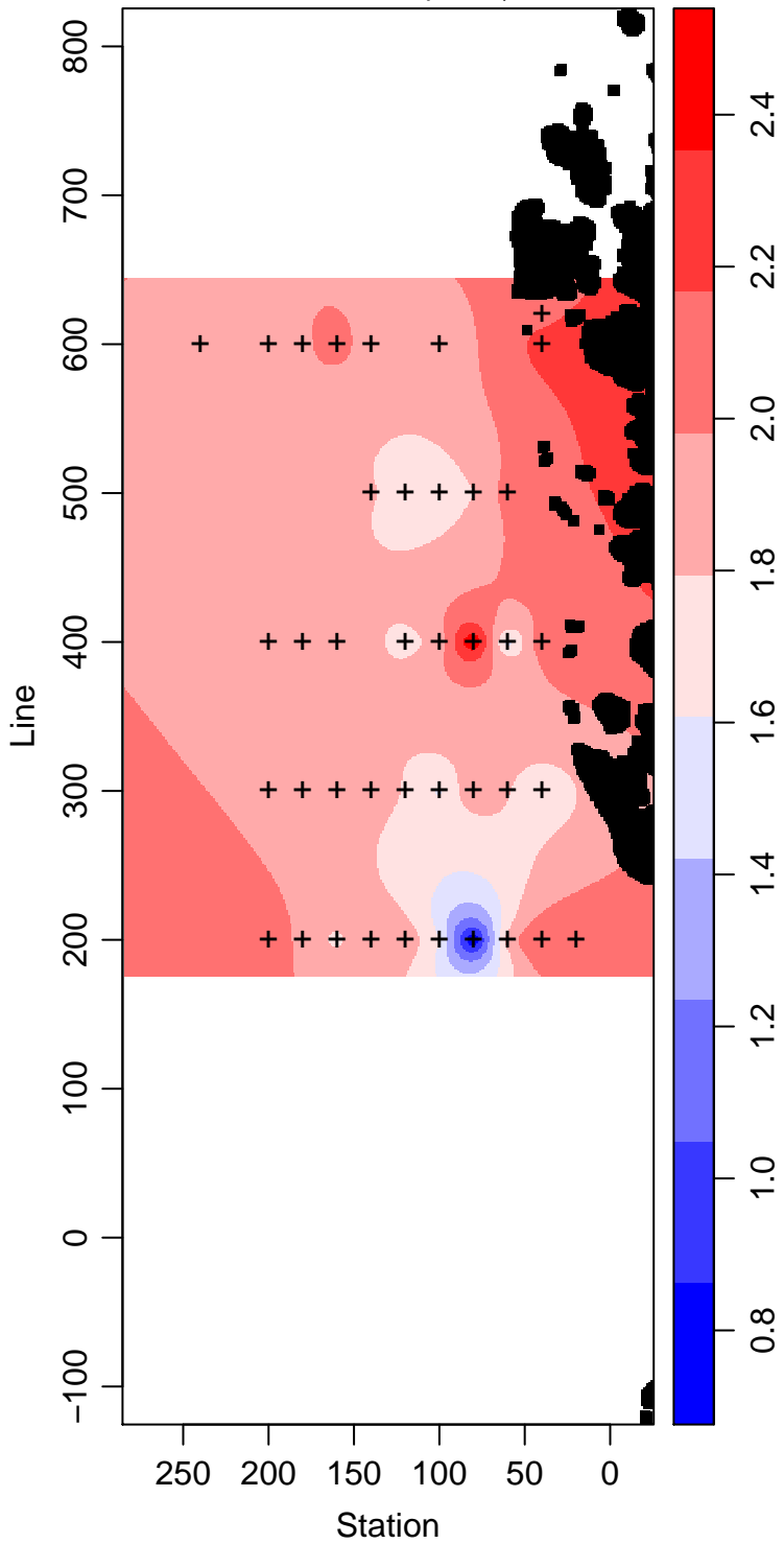
LMG05-01_30_Phosphate \mu\text{ mol L}^{-1}
