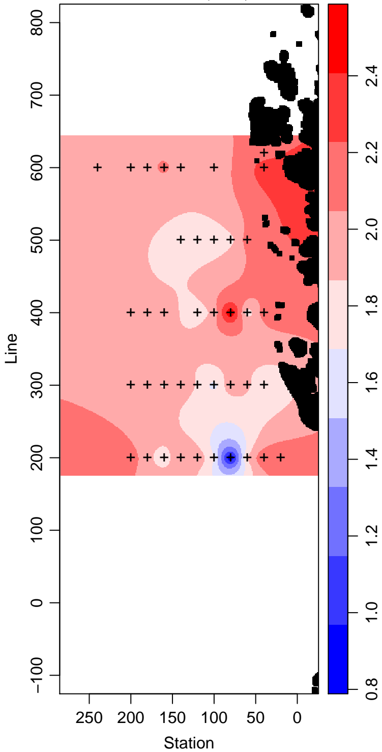
LMG05-01_35_Phosphate \mu\text{ mol L}^{-1}
