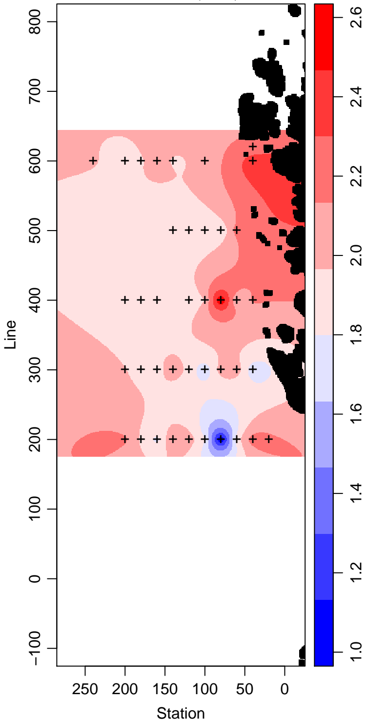
LMG05-01_40_Phosphate \mu\text{ mol L}^{-1}
