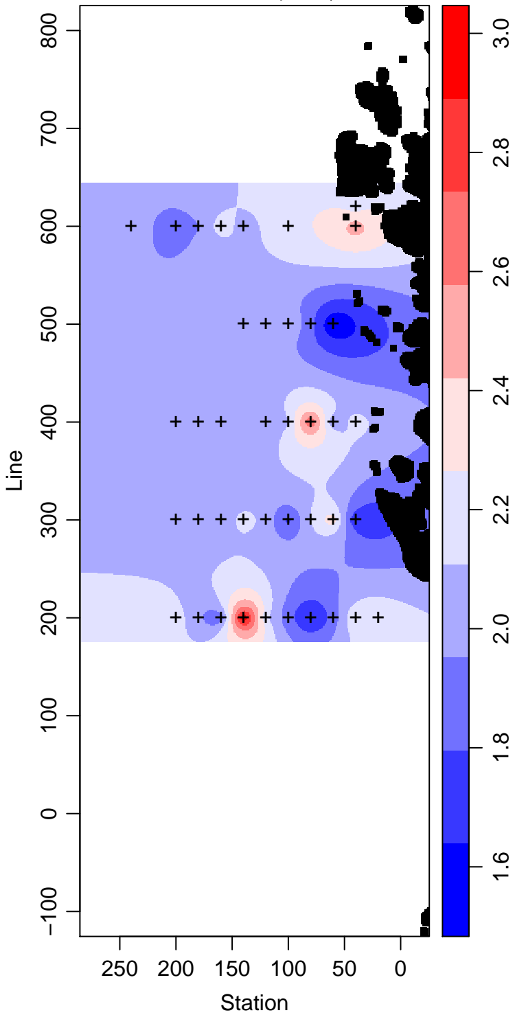
LMG05-01_50_Phosphate \mu\text{ mol L}^{-1}
