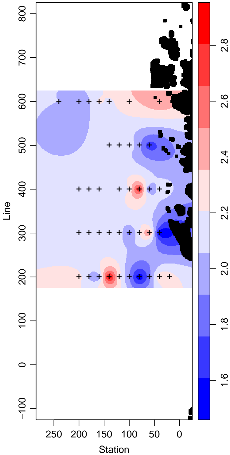
LMG05-01_60_Phosphate \mu\text{ mol L}^{-1}
