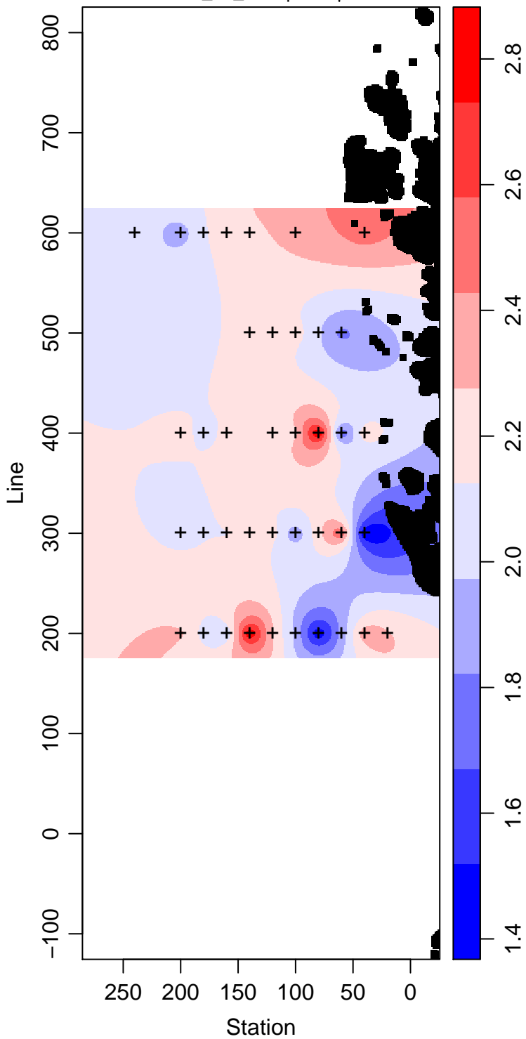
LMG05-01_65_Phosphate \mu\text{ mol L}^{-1}
