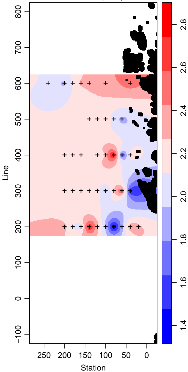
LMG05-01_70_Phosphate \mu\text{ mol L}^{-1}
