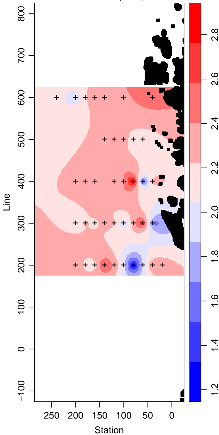
LMG05-01_80_Phosphate \mu\text{ mol L}^{-1}
