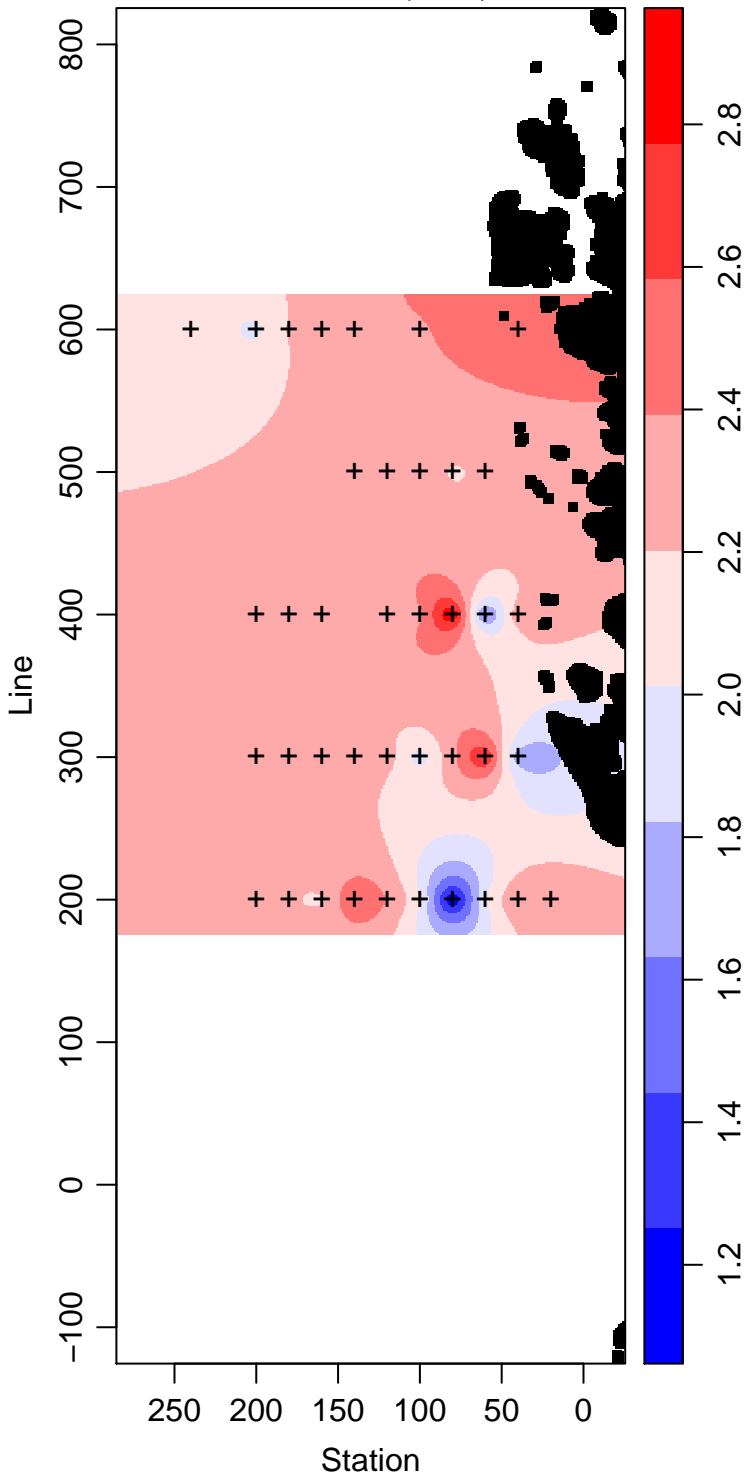
LMG05-01_85_Phosphate \mu\text{ mol L}^{-1}
