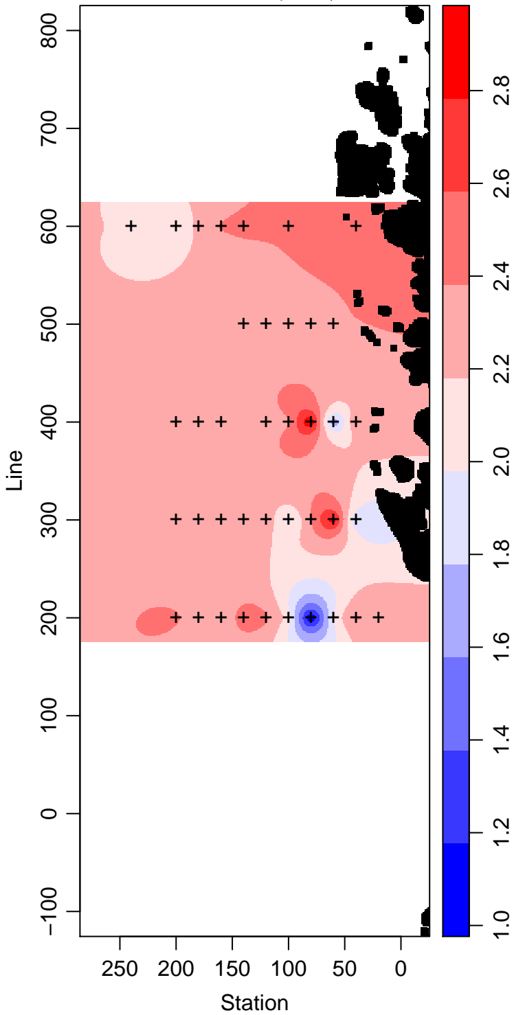
LMG05-01_90_Phosphate \mu\text{ mol L}^{-1}
