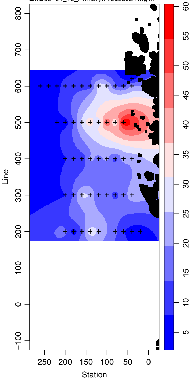
LMG05-01_15_Primary.Production mg m -3
