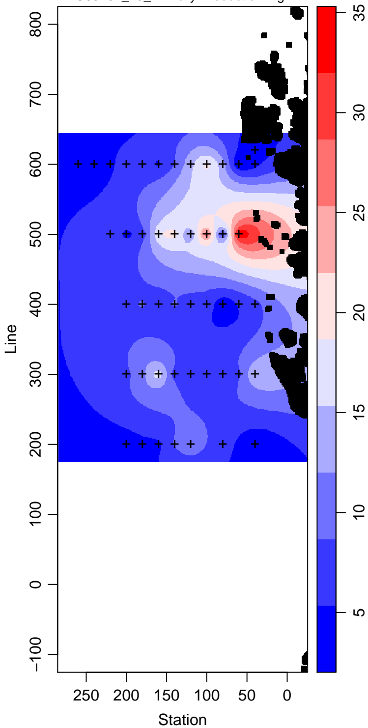
LMG05-01_25_Primary.Production mg m -3
