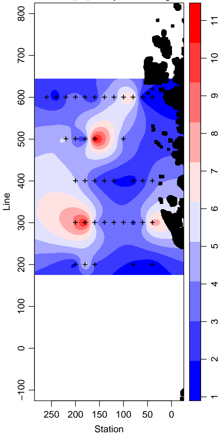
LMG05-01_45_Primary.Production mg m -3
