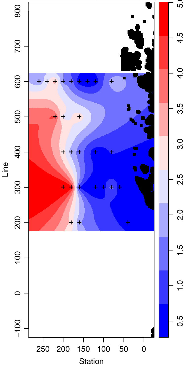
LMG05-01_70_Primary.Production mg m -3
