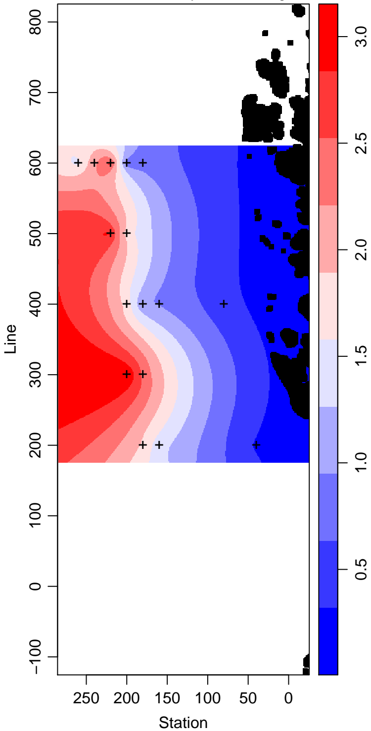
LMG05-01_80_Primary.Production mg m -3
