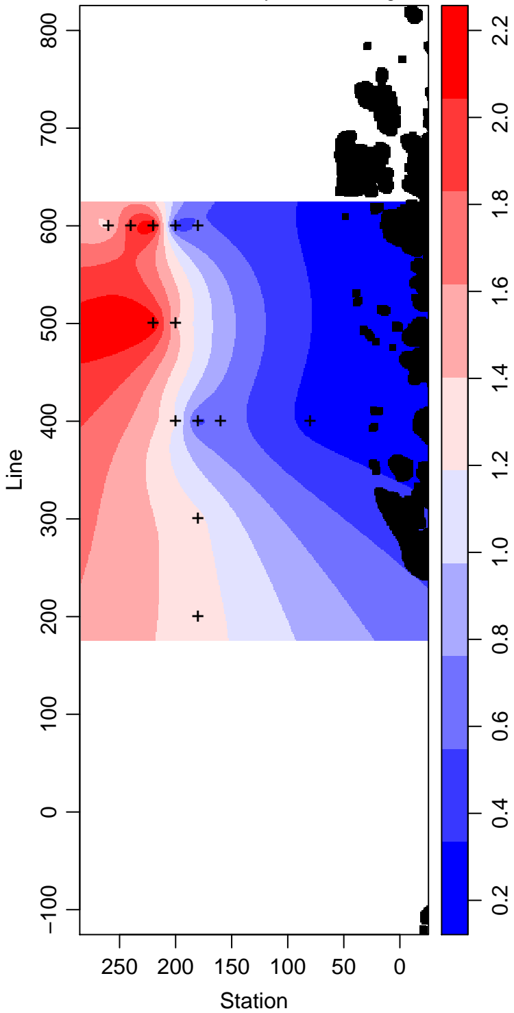
LMG05-01_85_Primary.Production mg m -3
