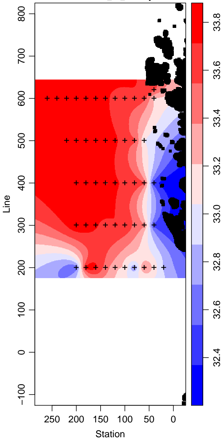
LMG05-01_10_Salinity
