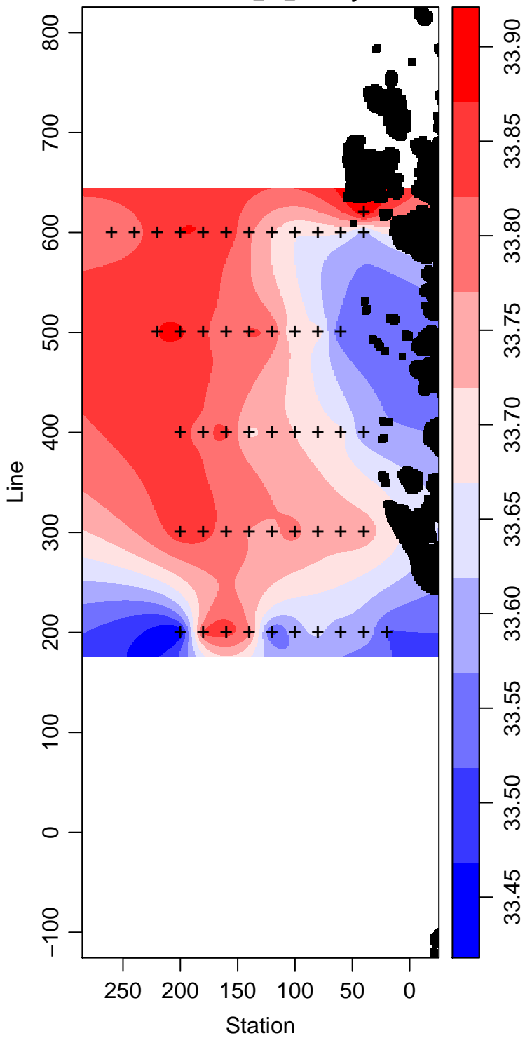
LMG05-01_30_Salinity
