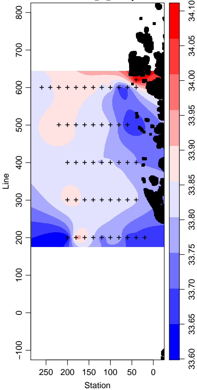
LMG05-01_45_Salinity
