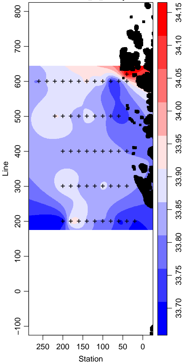
LMG05-01_50_Salinity
