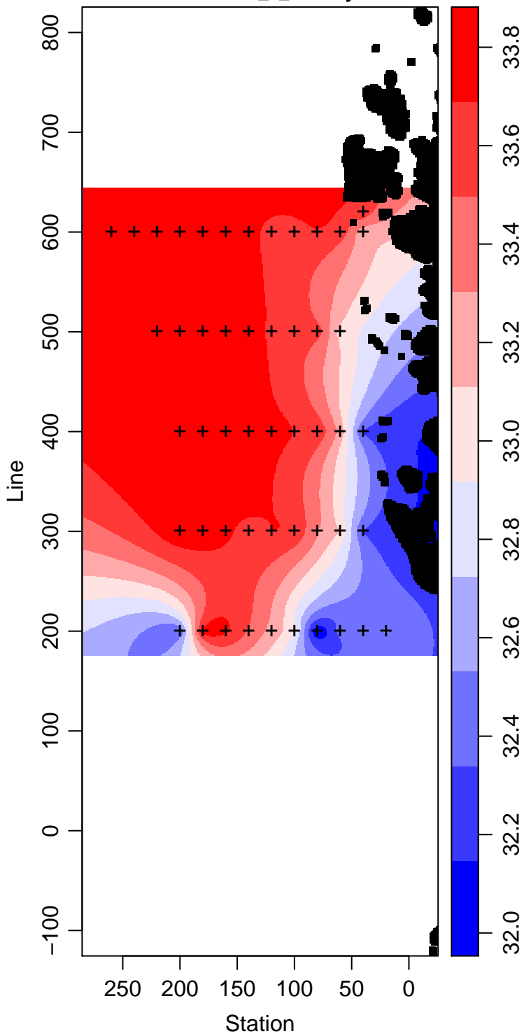
LMG05-01_5_Salinity
