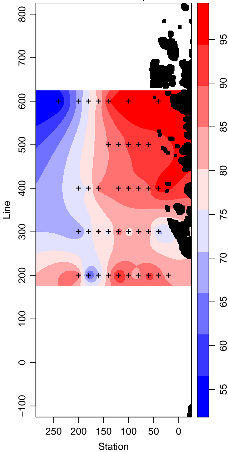
LMG05-01_100_Silicate \mu\text{ mol L}^{-1}
