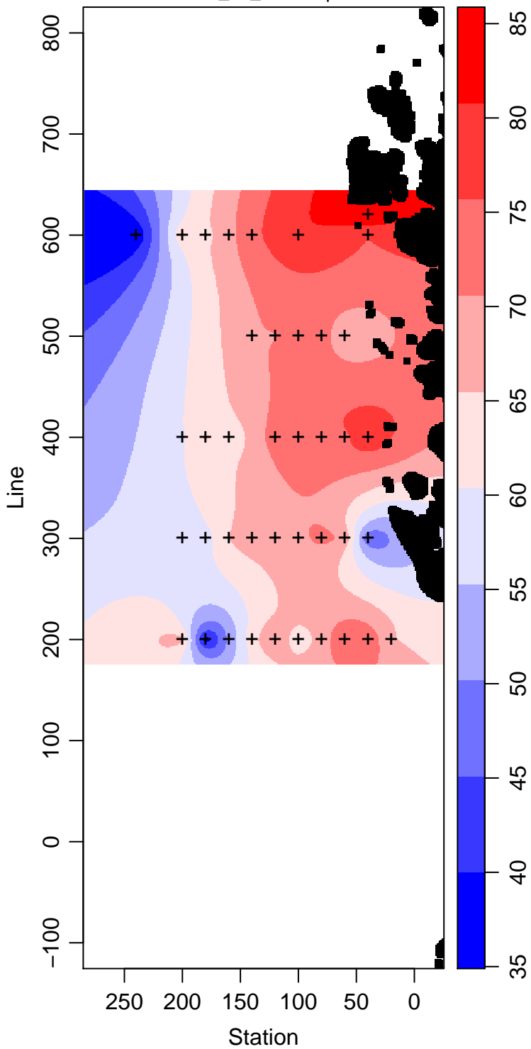
LMG05-01_10_Silicate \mu\text{ mol L}^{-1}
