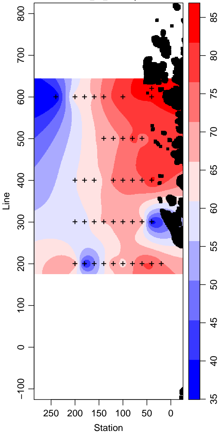
LMG05-01_15_Silicate \mu\text{ mol L}^{-1}
