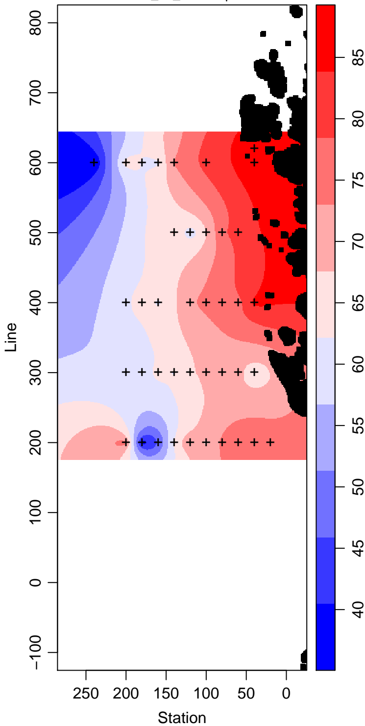
LMG05-01_25_Silicate \mu\text{ mol L}^{-1}
