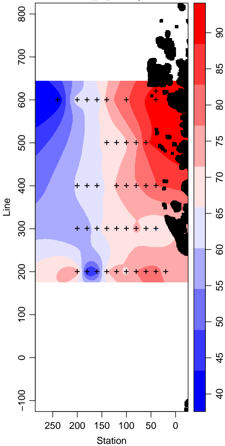
LMG05-01_35_Silicate \mu\text{ mol L}^{-1}
